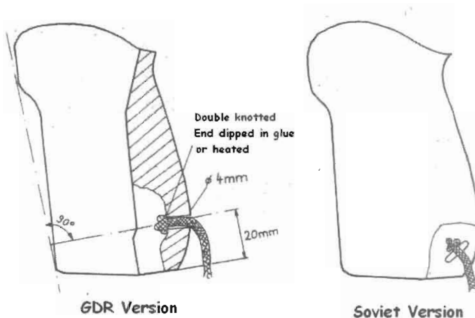
Picture 2.21 Attachment of the Lanyard to the Grip
