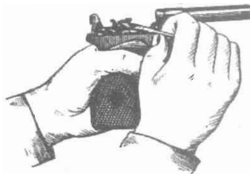
Picture 3.8 Removal of the hammer and slide lock from the frame
