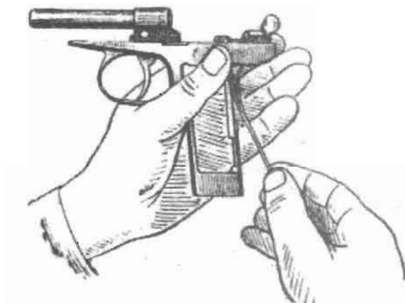
Picture 3.20 Attachment of the hammer spring to the frame
