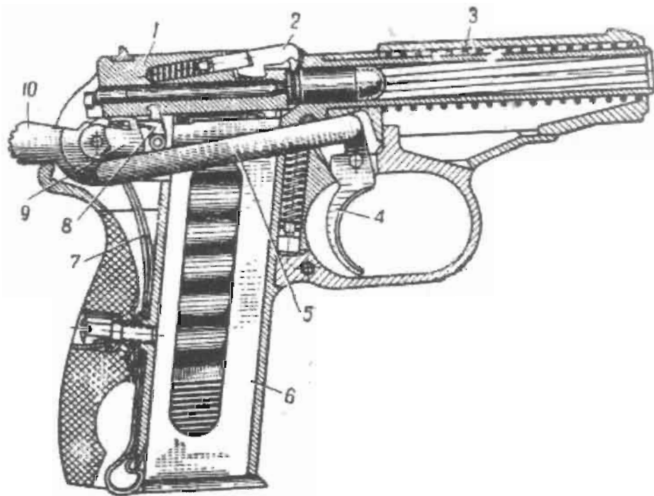
Picture 4.1 Position of Parts Prior to Firing
